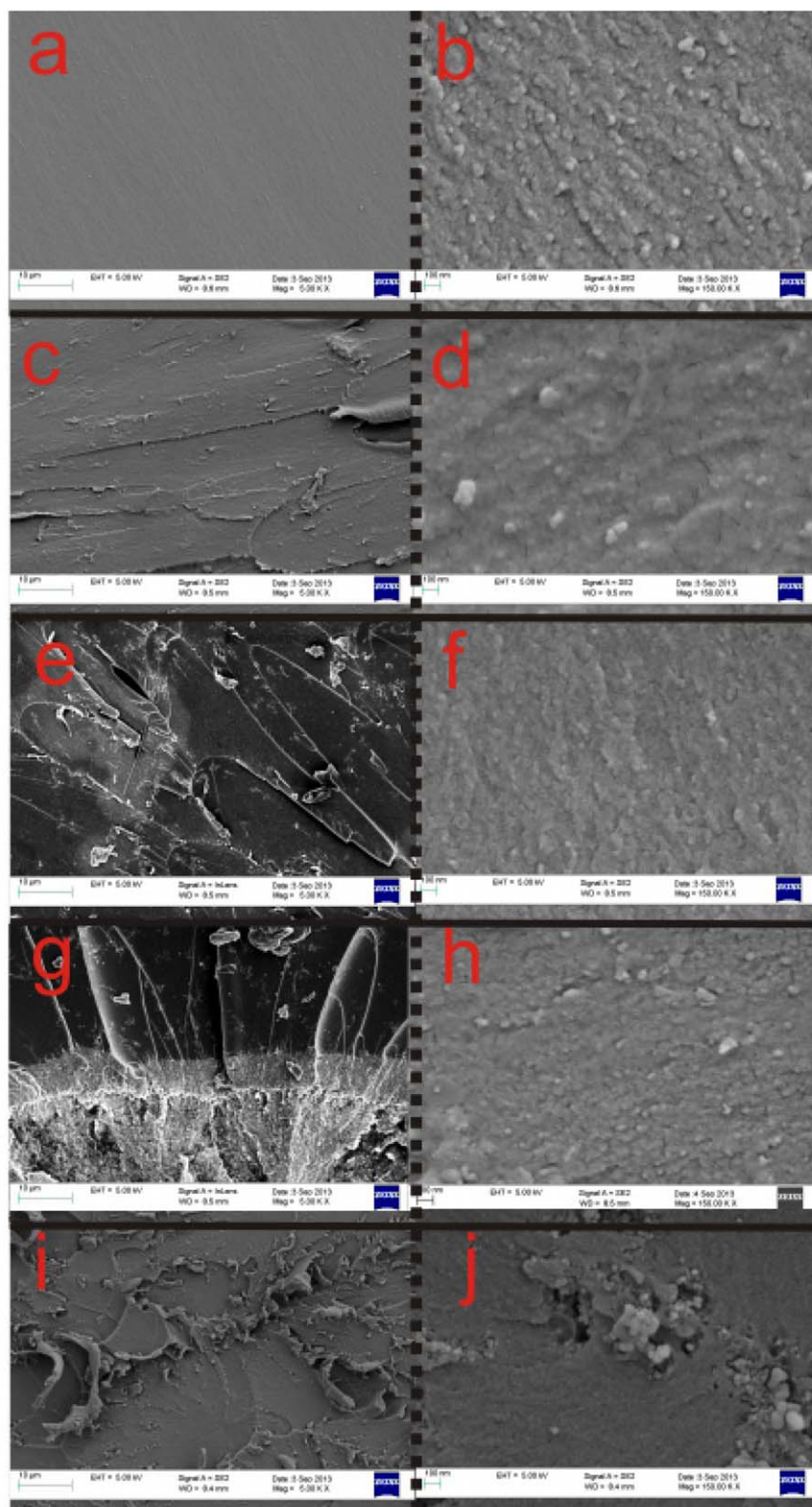
Figure 4. Fracture surface of (a) PUI 2 (11 kX), (b) PUI 2 (180 kX), Sil Polimix -PUI 2 1 wt % at (c) 11 kX, and (d) 180 kX, Sil Solvmix -PUI 2 1 wt % at (e) 11 kX, and (f) 180 kX, Sil Isopol -PUI 2 1 wt % at (g) 11 kX and (h) 180 kX, Sil Solvmix -PUI 2 1 wt % at (i) 11 kX and (j) 180 kX. [Color figure can be viewed in the online issue, which is available at wileyonlinelibrary.com .]
