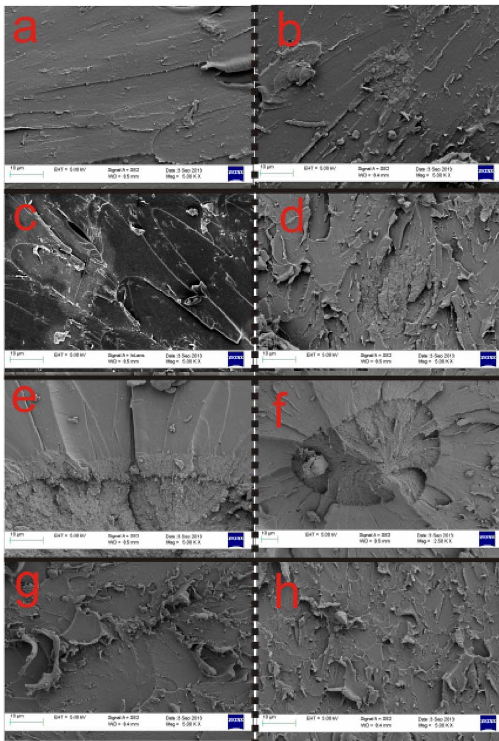
Figure 5. Fracture surface of (a) Sil Polmix -PUI 2 1 wt %, (b) Sil Polmix -PUI 2 2 wt %, (c) Sil Isomix -PUI 2 1 wt %, (d) Sil Isomix -PUI 2 4 wt %, (e) Sil Isopol -PUI 2 1 wt %, (f) Sil Isopol -PUI 2 4 wt %, (g) Sil Solvmix -PUI 2 1 wt %, and (h) Sil Solvmix -PUI 2 4 wt %. [Color figure can be viewed in the online issue, which is available at wileyonlinelibrary.com .]
