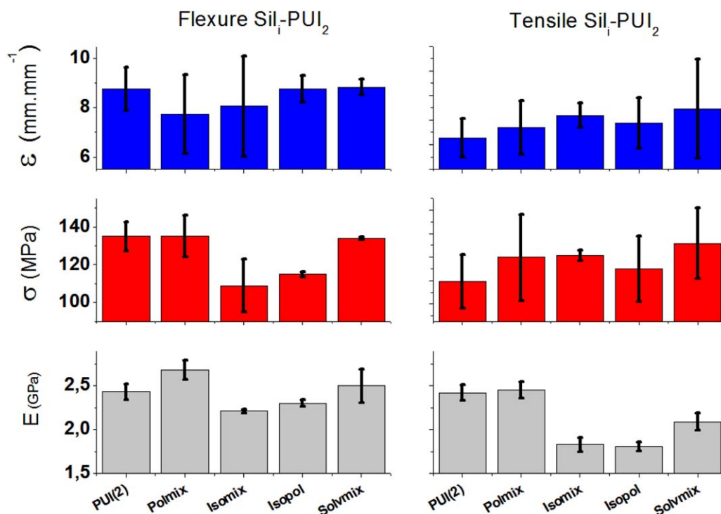
Figure 8. Tensile and Flexural mechanical properties as a function of processing route for the NC prepared at a fixed NS concentration of 1 wt %. [Color figure can be viewed in the online issue, which is available at wileyonlinelibrary.com .]
