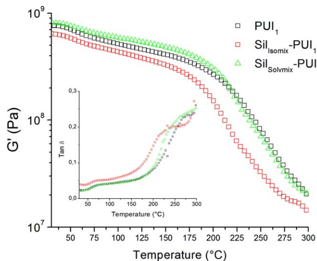
Figure 13. Elastic shear modulus ( G' ) and damping factor ( \text{Tan } \delta ) as a function of temperature for the PUI 1 , Sil Isomix -PUI 1 1 wt %, and Sil Solvmix -PUI 1 1 wt %. [Color figure can be viewed in the online issue, which is available at wileyonlinelibrary.com .]
