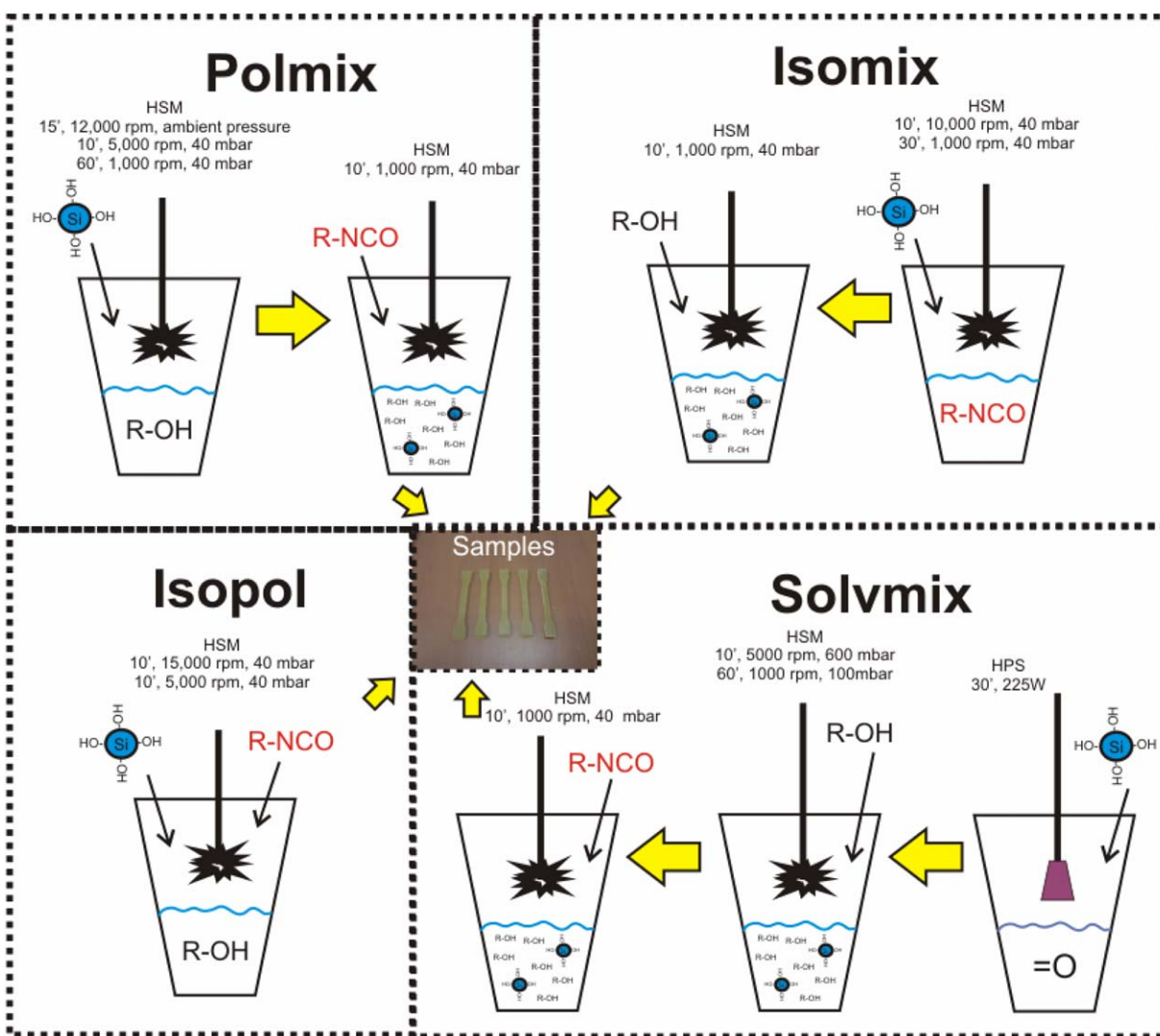
Figure 1. Processing routes used in this work to obtain \text{Si}_f\text{-PUI}_x\text{ NC} . [Color figure can be viewed in the online issue, which is available at wileyonlinelibrary.com .]
