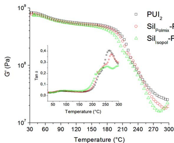
Figure 14. Elastic shear modulus ( G' ) and damping factor ( \text{Tan } \delta ) as a function of temperature for the PUI 2 , Sil Polmix -PUI 2 1 wt %, and Sil Isopol -PUI 2 1 wt %. [Color figure can be viewed in the online issue, which is available at wileyonlinelibrary.com .]
